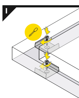
spojka LINEA-IN20 90° LINEA-IN20 connector 90 deg
